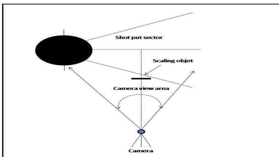
Figure 1: Camera setup for two-dimensional quantitative analysis
